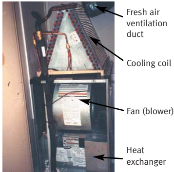
Inside a typical electric furnace closet
