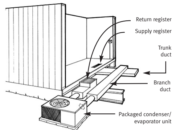
Packaged system air conditioner
